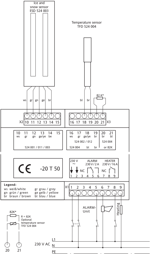
Connection diagram 2: Ice detector connection with ESD 524 003 and TFD 524 004 sensors for gutter heating.
