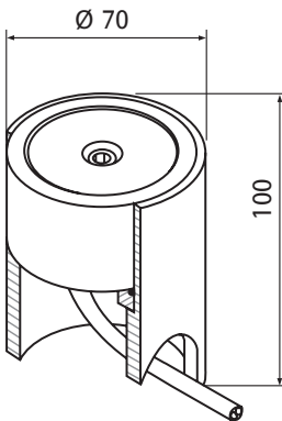
ESF 524 011 with FAG 524 111 sensor housing
